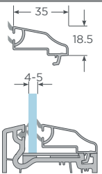
Junquillo 4-5mm - S60
