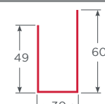
Ref. Hoja Puerta S60 1.5mm - TC PL-S60-TC-HPF-15
