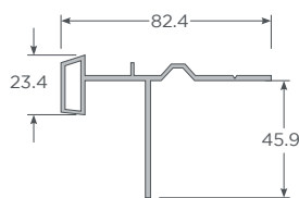
New Aleta Siding
