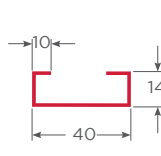
Ref. marco corredera 1.2mm - TC PL-SLD-TC-MCA-12
