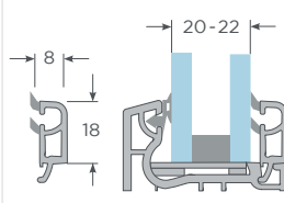
Junquillo 20-22mm Corredera
