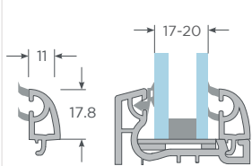
Junquillo 17-20mm Corredera
