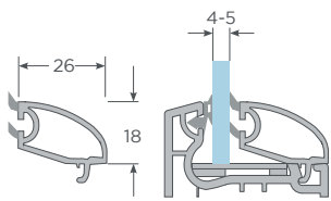
Junquillo 4-5mm Corredera
